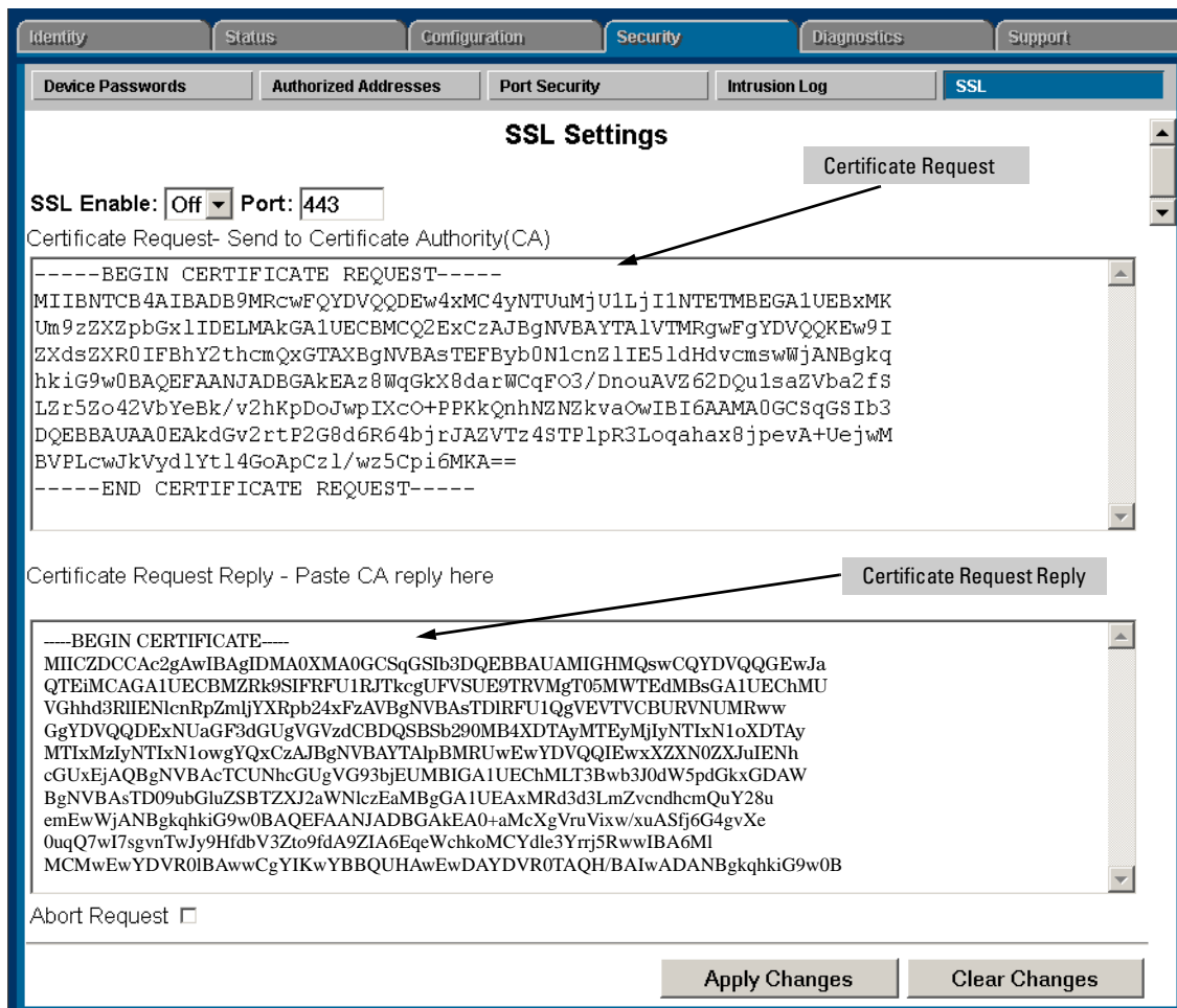
Figure 8-7. Request for Verified Host Certificate Web Browser Interface Screen
